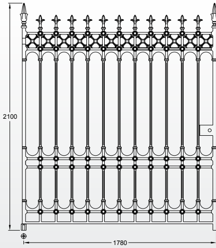
Stirling driveway gate (12 x 7ft pair, 510kg)
