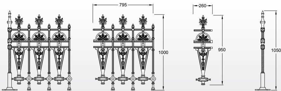
Gilberton railing panel & Gilberton intermediate railing post
