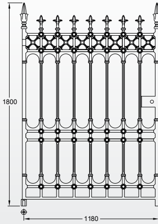
Stirling pedestrian gate (4 x 6ft, 178kg)
