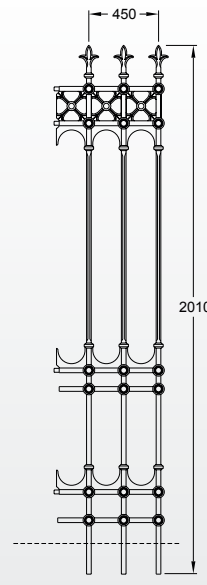
Stirling full height railing panel (24kg)
