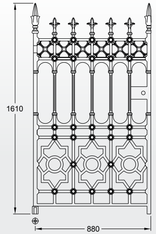
Stewart pedestrian gate (3ft, 117kg)
