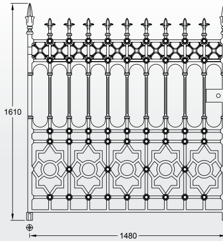
Stewart driveway gate leaf (10ft pair, 370kg)
