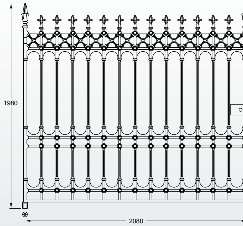
Stirling driveway gate (14 x 6.5ft pair, 620kg)
