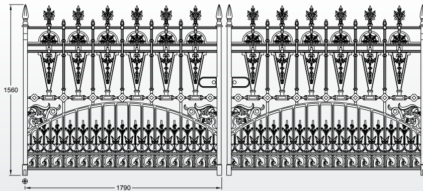
Gilberton driveway gate leaf (12ft pair, 464kg)
