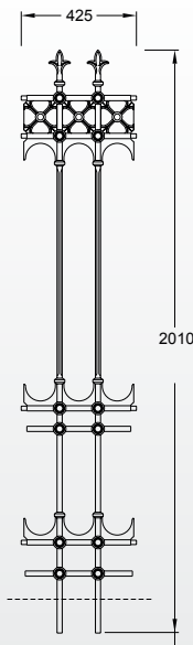
Stirling full height joining panel (18kg)
