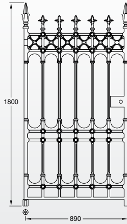
Stirling pedestrian gate (3 x 6ft, 178kg)
