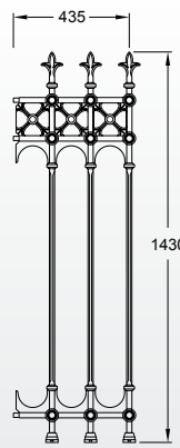
Stirling half height railing panel (33kg)
