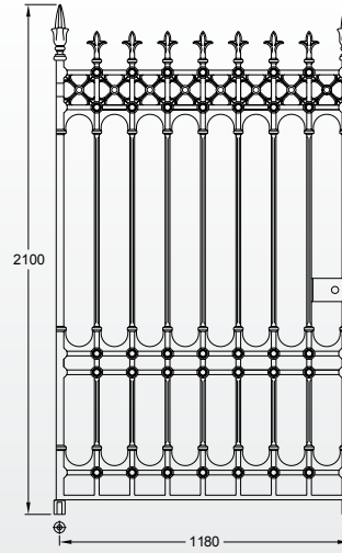
Stirling pedestrian gate (4 x 7ft, 178kg)
