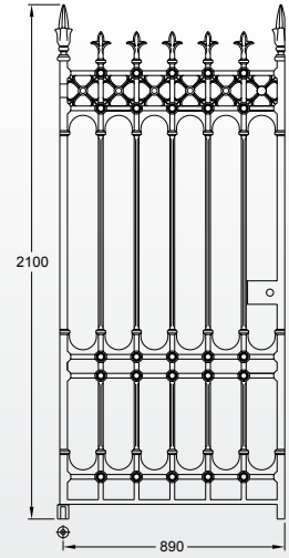
Stirling pedestrian gate (3 x 7ft, 142kg)
