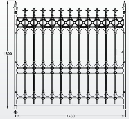
Stirling driveway gate (12 x 6ft pair, 400kg)
