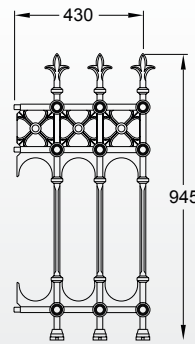
Stewart half height railing panel (20.5kg)
