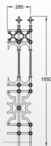
Stewart full height railing panel (24kg)
