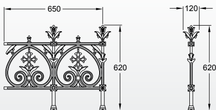
Terrace railing panel(36.5kg)
